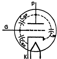
Interelectrode capacitances in a triode.
